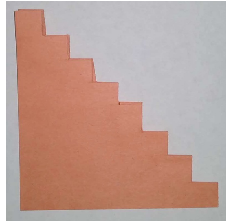
iteration 3
