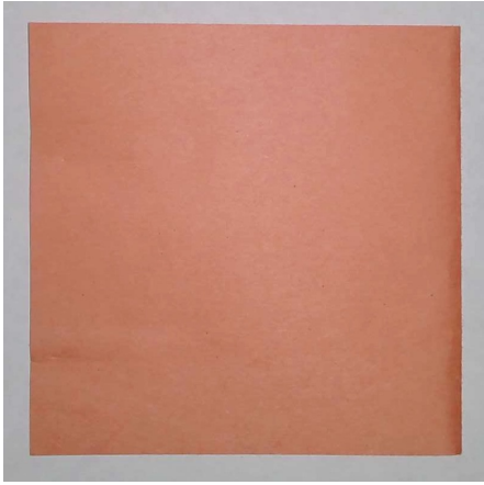
iteration 0
