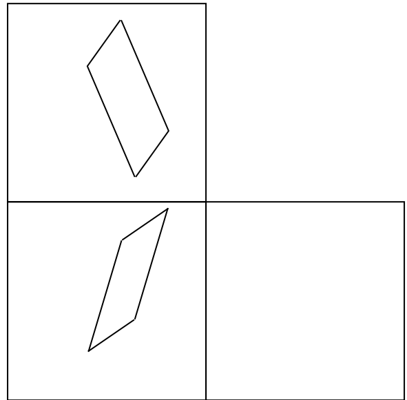
Problem #2 (A square)
