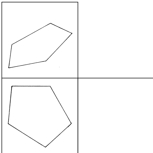
Problem #3 (A regular pentagon)
