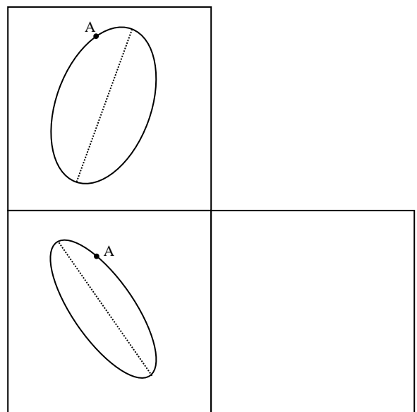
Problem #4 (A circle)
