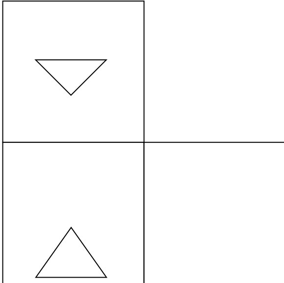
Problem #1 (An equilateral triangle)
