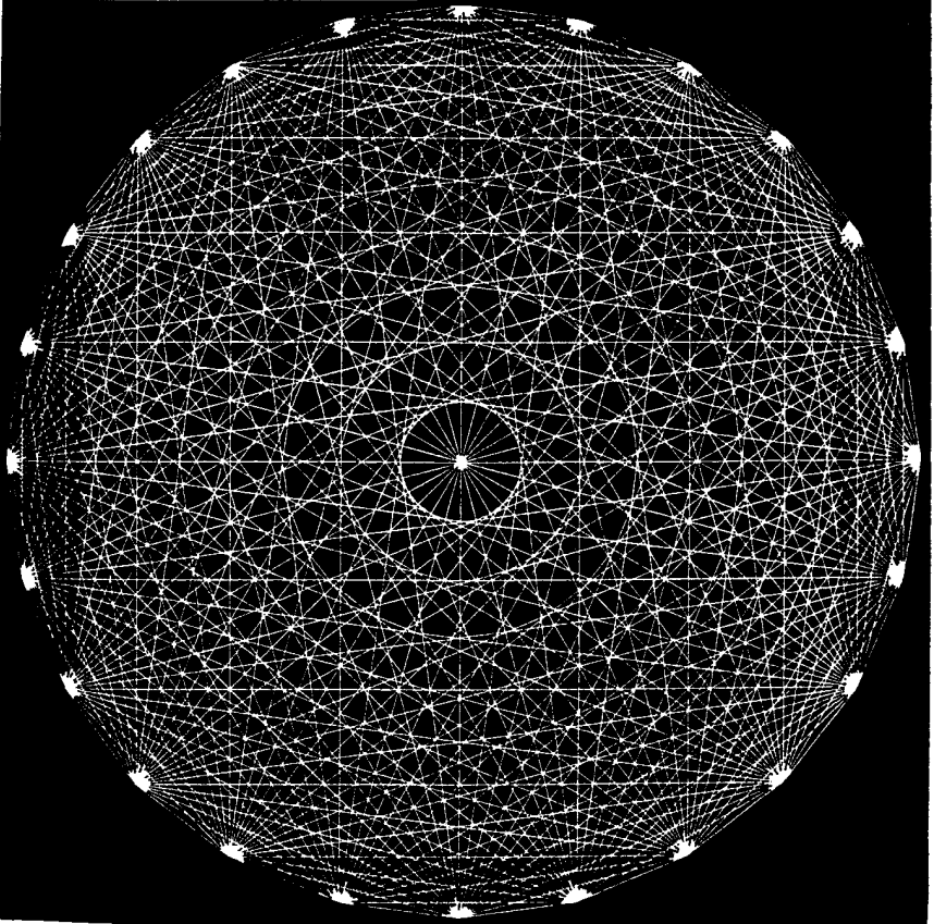
The 24-division with All of its Diagonals
